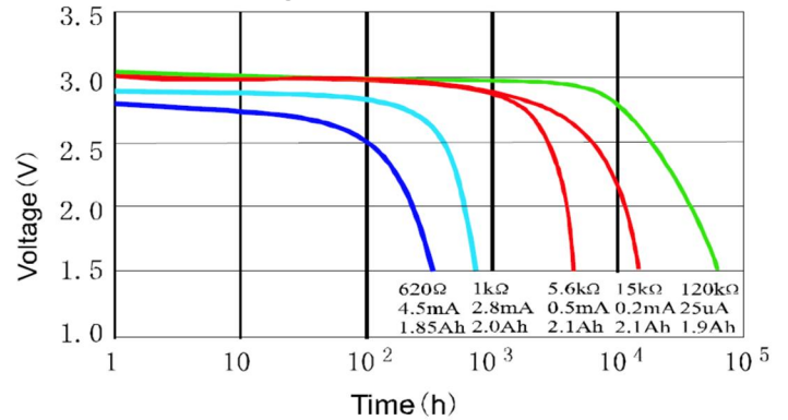
Capacity vs Current
