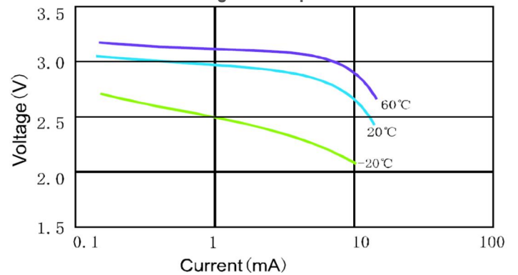
Discharge Characteristics after Storage
