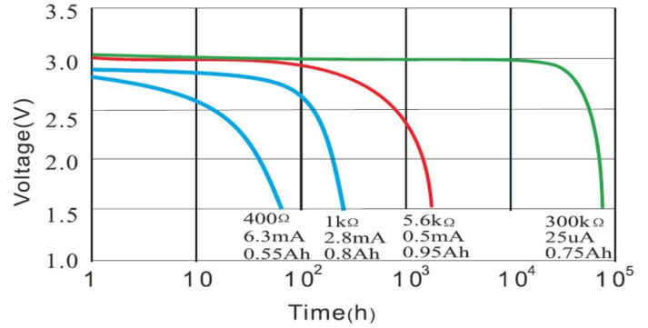
Capacity vs Current
