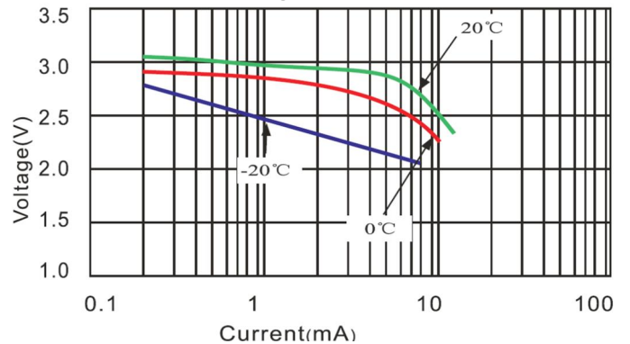
Discharge Characteristics after Storage
